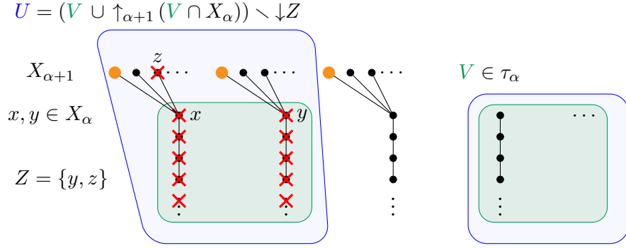
FIGURE 3. A member of \mathcal{S}_{\alpha+1} of the form described in condition (iii). For each v \in X_{\alpha} we coloured in orange the corresponding element v^+ of X_{\alpha+1} . Furthermore, we coloured in green the set V \in \tau_{\alpha} . Lastly, Z = \{y, z\} is a finite subset of P_{\alpha} \cup \mathcal{S}_{\alpha+1} . Then the set U = (V \cup \uparrow_{\alpha+1}(V \cap X_{\alpha})) \setminus \downarrow Z is obtained by considering the blue shape and removing the elements crossed in red from it.
